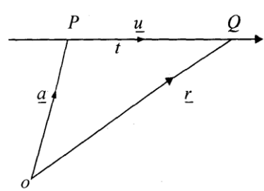
Fig.(2) : vector fields
