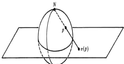
Fig. (1): the diffeomorphism
