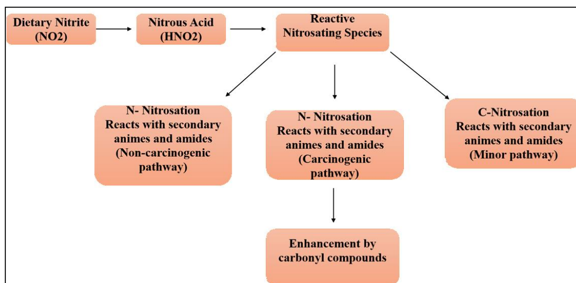
Figure 1: Formation and competing fates of nitrosating species
